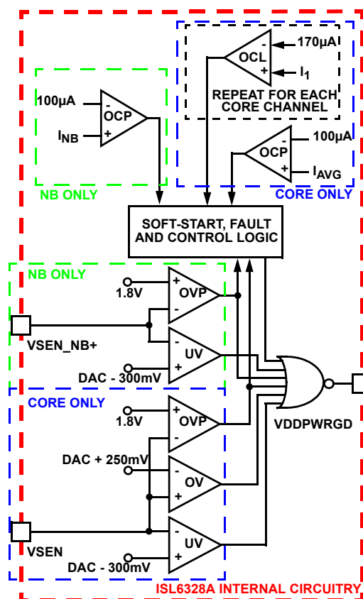
FIGURE 13. POWER-GOOD AND PROTECTION CIRCUITRY
