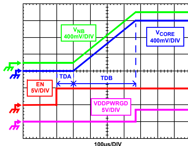
FIGURE 11. SOFT-START WAVEFORMS
