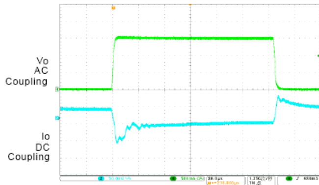
8. Load Transient Response
