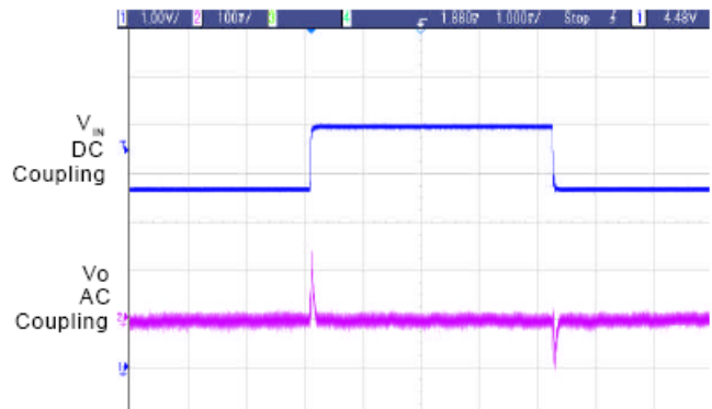
9. Line Transient Response
