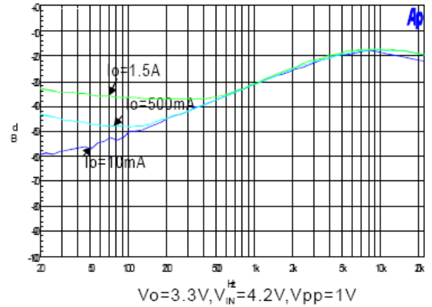
7. Ripple Rejection vs Frequency
