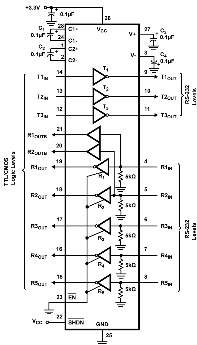
ICL3241
