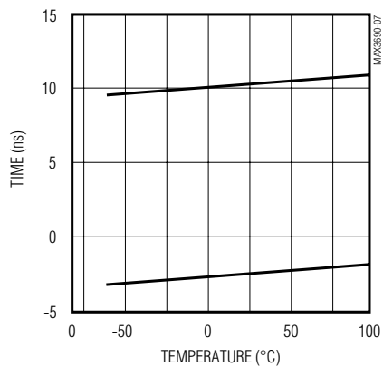
ALLOWED PCLK0 to PCLK1 SKEW vs. TEMPERATURE
