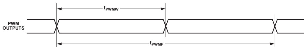
Figure 25. PWM Timing
