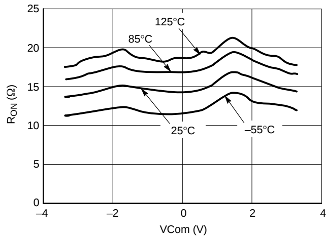
Figure 9. Typical On Resistance V_{CC} = 3.0 V, V_{EE} = -3.0 V
