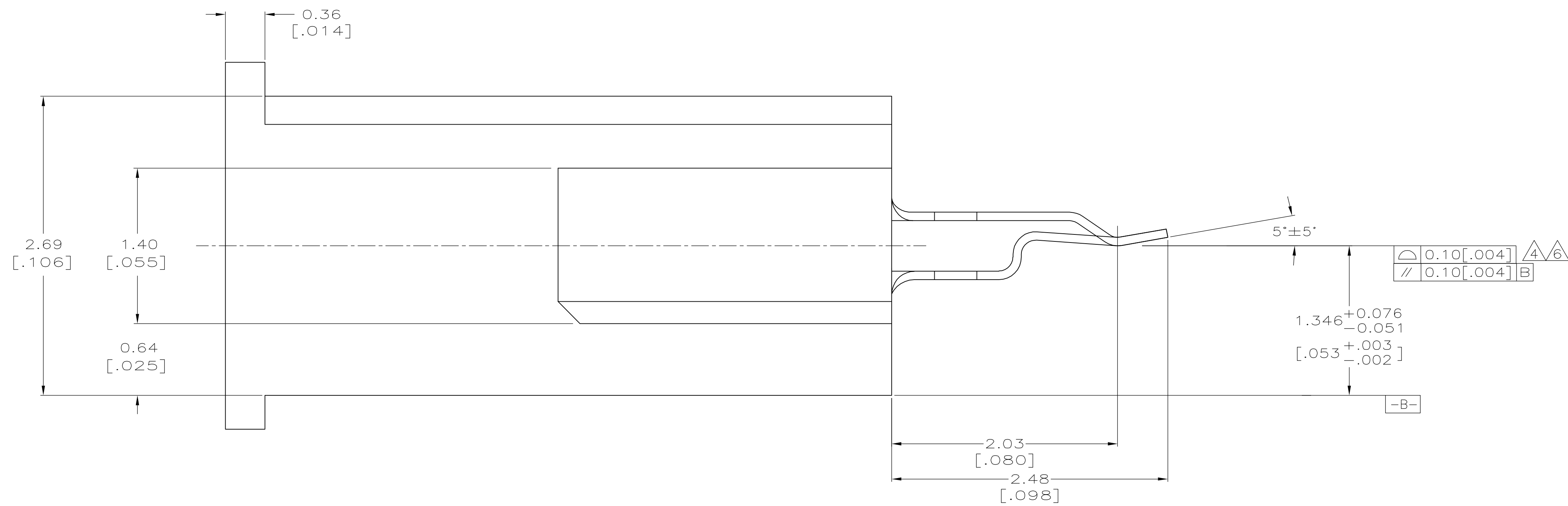
VIEW Z-Z SCALE 40:1
