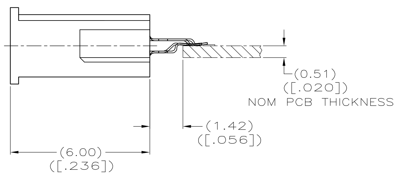
RECOMMENDED PC BOARD LOCATION SCALE: 10:1
