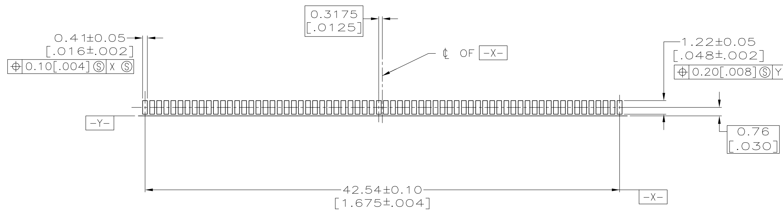
RECOMMENDED PC BOARD LAYOUT
