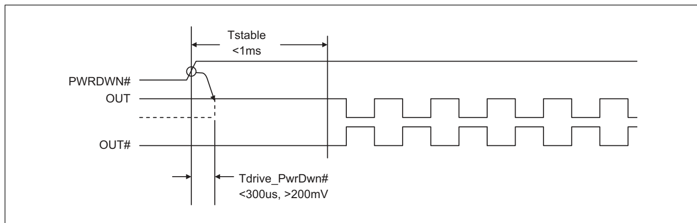
Figure 2. Power down de-assert sequence
