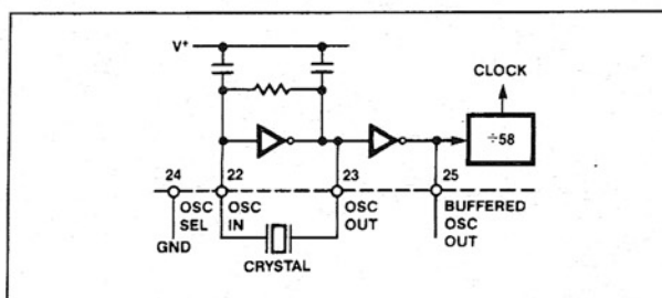
Figure 7. Crystal Oscillator
