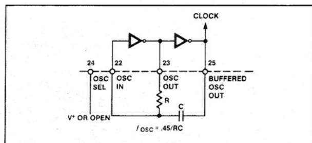
Figure 6. RC Oscillator
