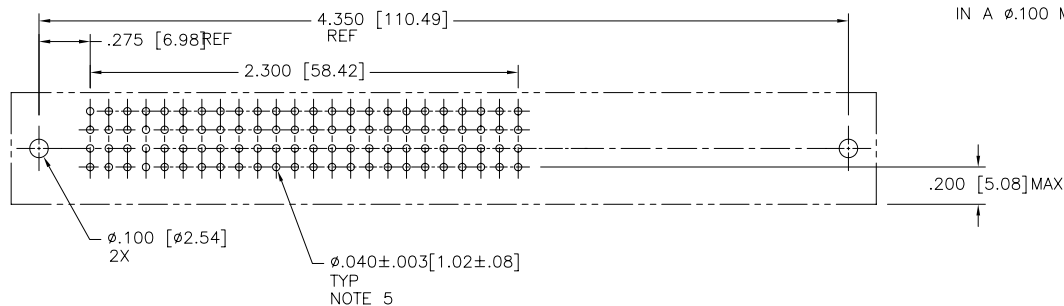
RECOMMENDED PCB LAYOUT (ALL HOLES LOCATED ON .100 [2.54] GRID UNLESS OTHERWISE SPECIFIED)
