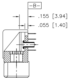
SECTION U-U
