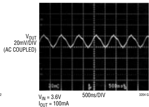
Output Ripple
