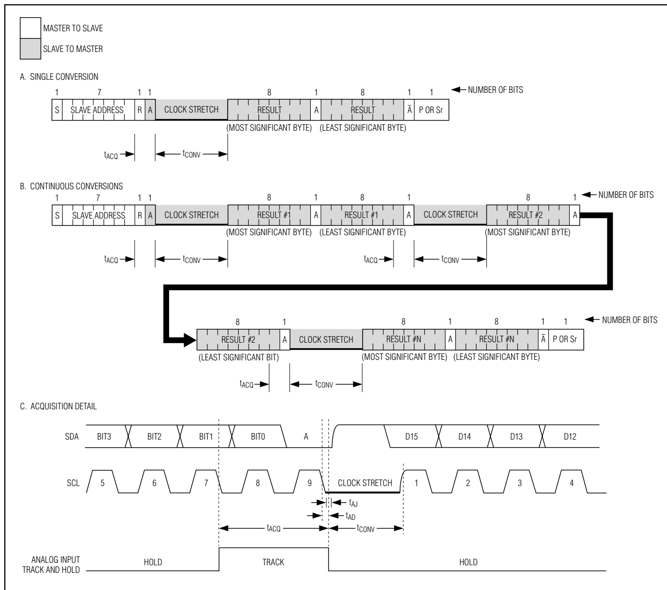
Figure 11. Read Cycle
