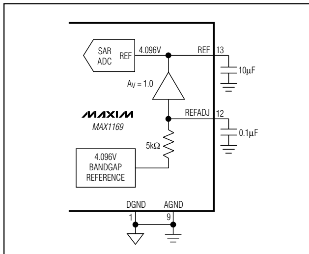
Figure 12. Internal Reference
