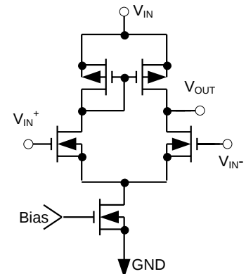
Figure 5 Error amplifier
