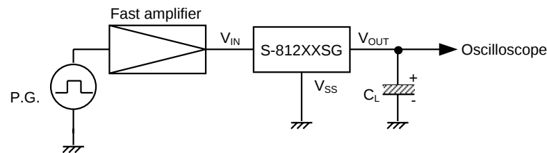
Figure 8 Measuring circuit
