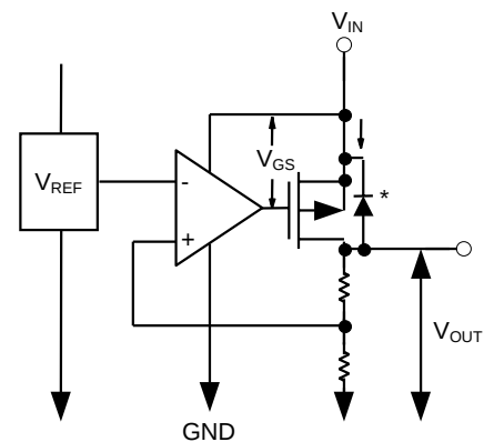
Figure 5 Error amplifier
