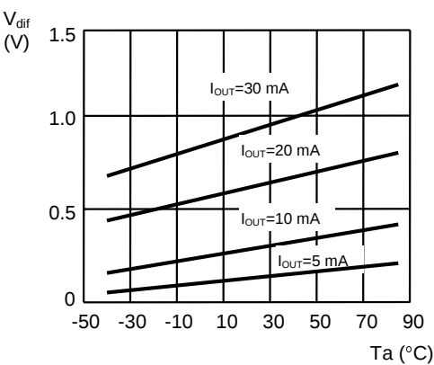
7.6 S-81235SG series
