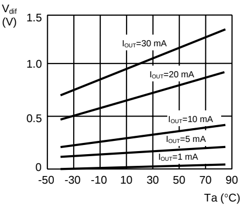
7.4 S-81225SG series
