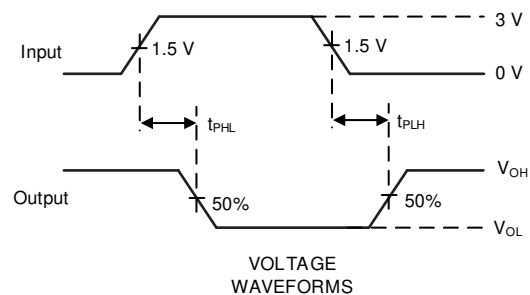
Figure 8-3. Receiver Propagation Delay Times
