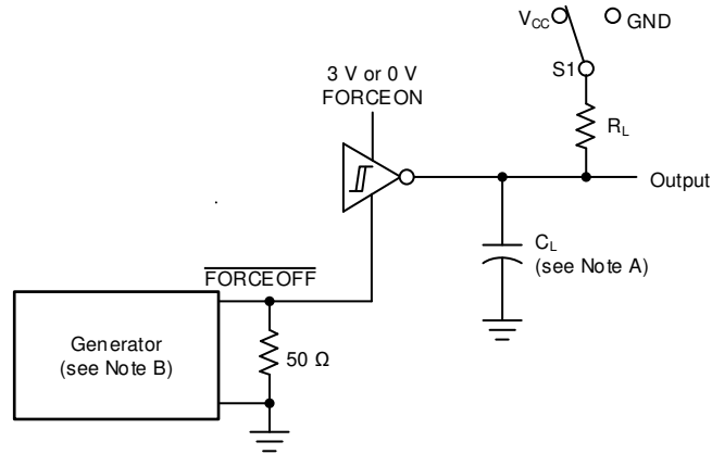
TEST CIRCUIT
