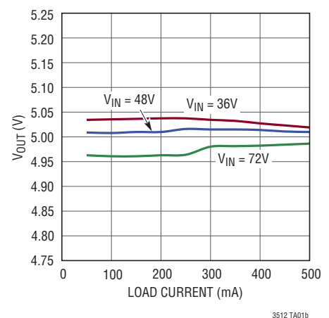
Output Load and Line Regulation
