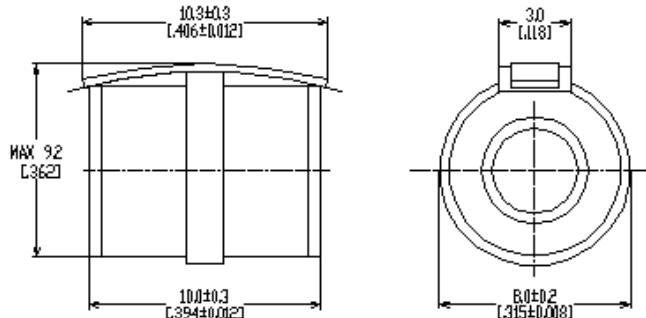
No Leads with-FT (GTCN38-XXXM-R10-FT)
