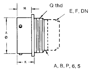
Crimp KPSE00/MS3120
