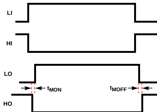
FIGURE 4. DELAY MATCHING
