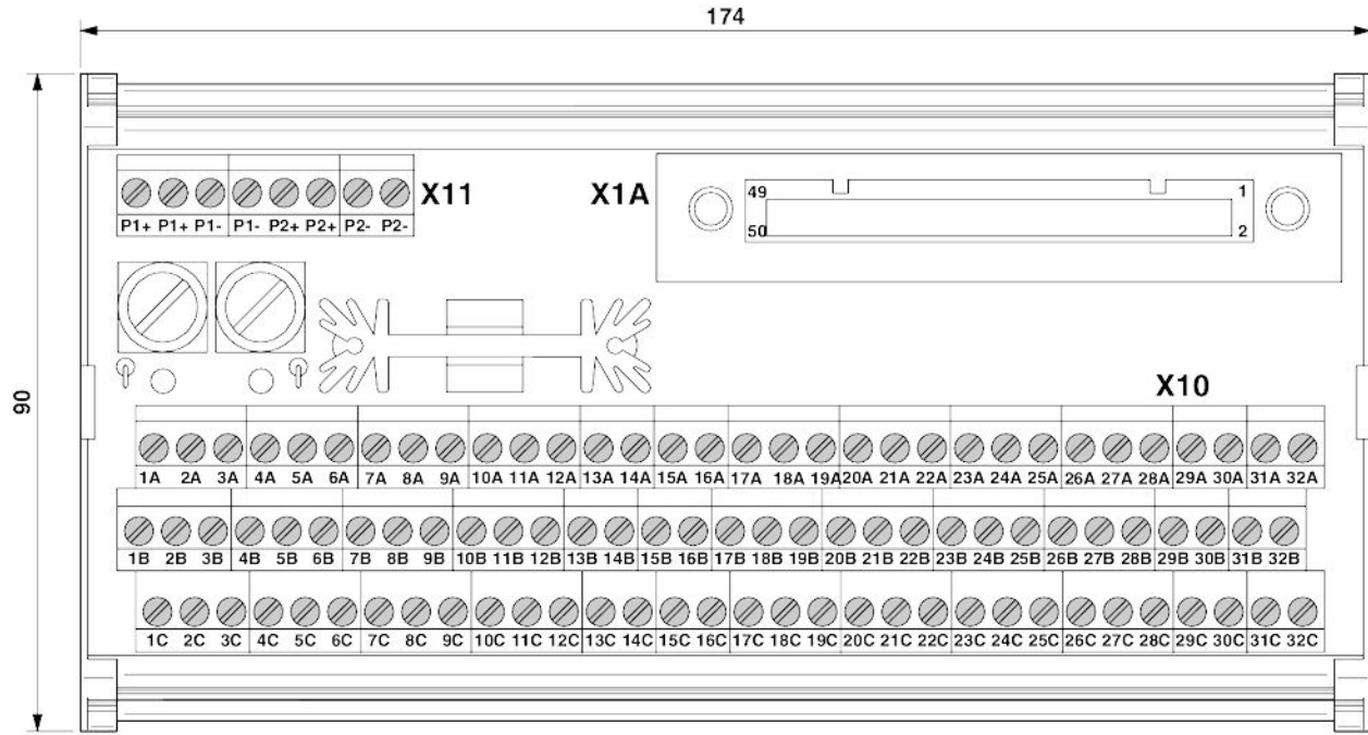
Dimensional drawing
