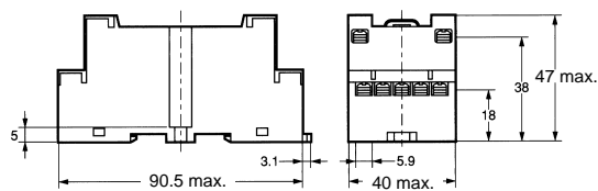
With Safety Relay Mounted
