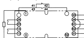
Terminal Installation/Internal Connection Diagram (Top View)
