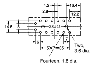
Cross-section of Mounting Holes
