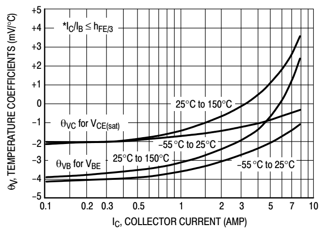
Figure 5. Temperature Coefficients
