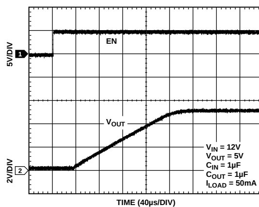
Figure 18. Start-Up Time
