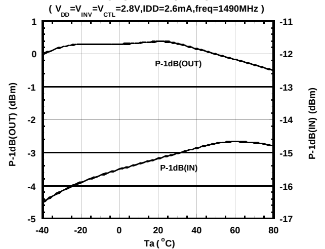
P-1dB(IN),P-1dB(OUT) vs. Ta
