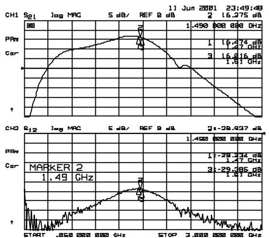
S 21 , S 12
