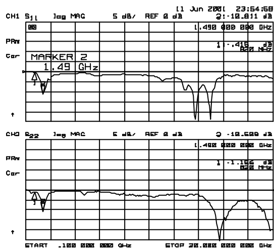
S11, S22
