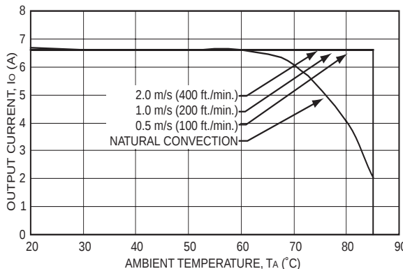
Figure 45. Derating Curves for HW006A6A1 (VO = 5.0 V) in Transverse Orientation (VI = 48 Vdc).
