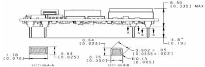
Bottom View
