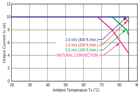
Figure 44. Derating Curves for HW010A0F1 (VO = 3.3 V) in Transverse Orientation (VI = 48 Vdc).
