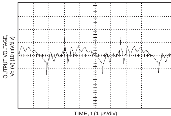
Figure 15. Output Ripple Voltage ( I_O = I_{O, \text{max}} ).
