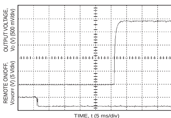
Figure 24. Start-up from Remote On/Off ( I_O = I_{O, \text{max}} ).
