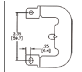
Front Bracket
