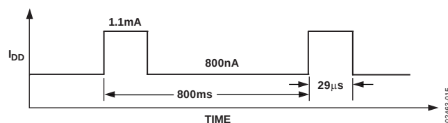
Figure 15. Mode 2 Power Dissipation
