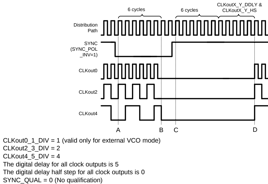
Figure 13. Clock Output Synchronization Using the SYNC Pin (Active Low)
