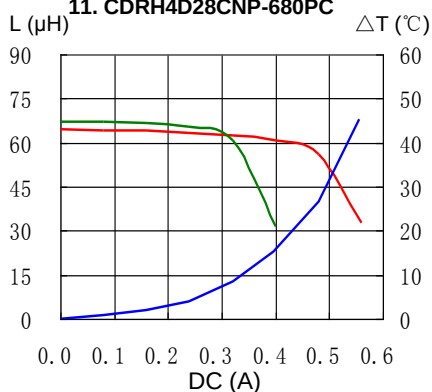
11. CDRH4D28CNP-680PC
