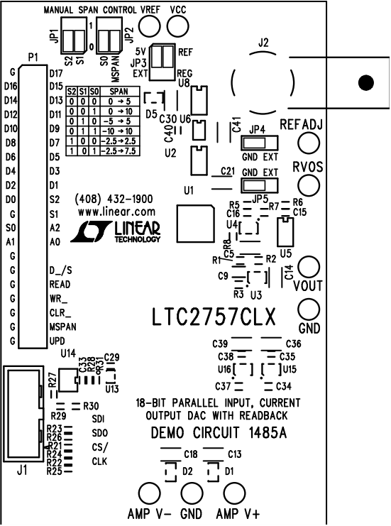
Top Silkscreen
