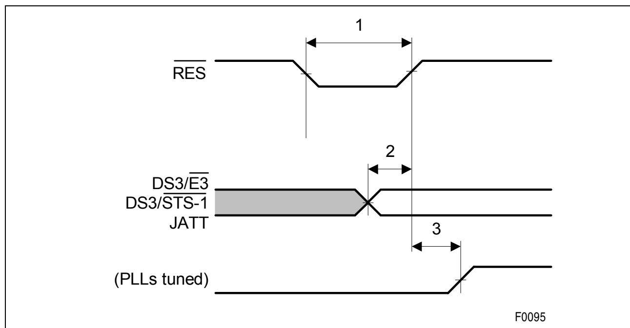
Figure 18 Reset Timing
