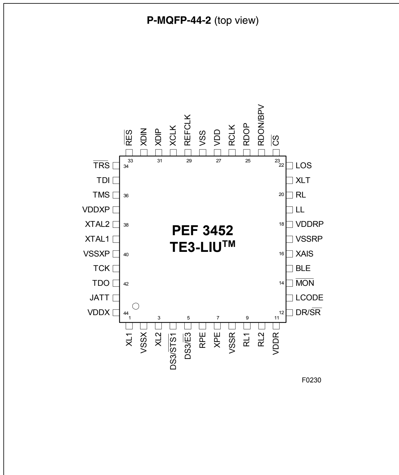
Figure 5 Pin Configuration
