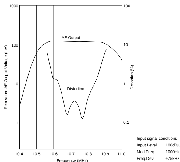
Frequency Characteristics
