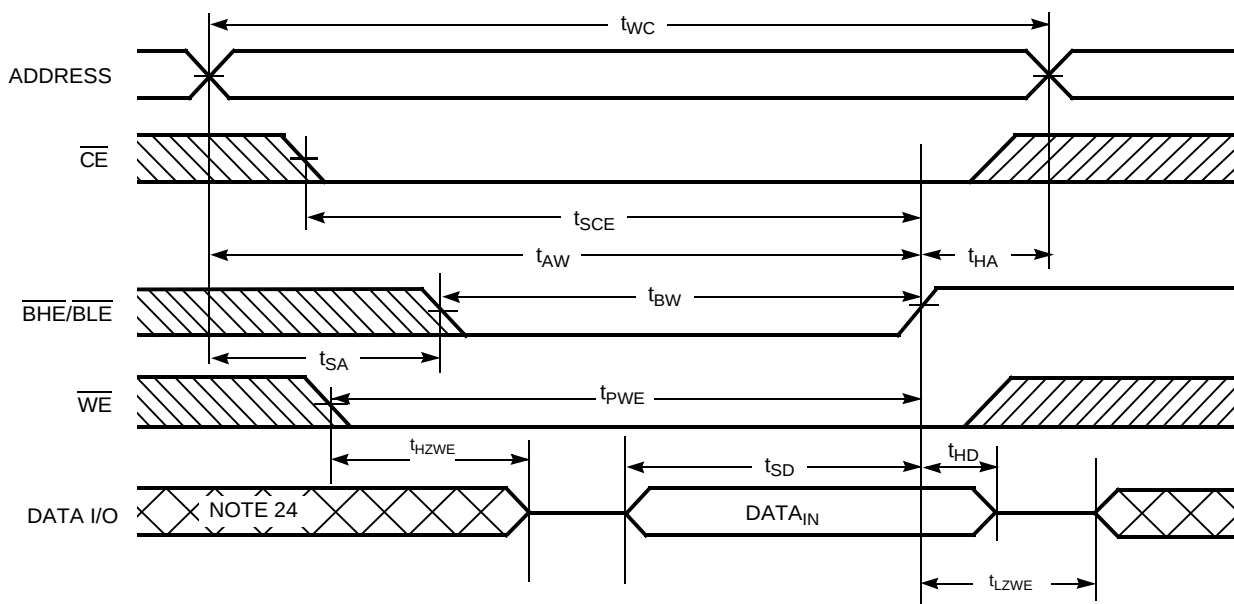
Figure 10. Write Cycle No. 4 ( \overline{\text{BHE/BLER}} controlled, \overline{\text{OE}} LOW) [23]
