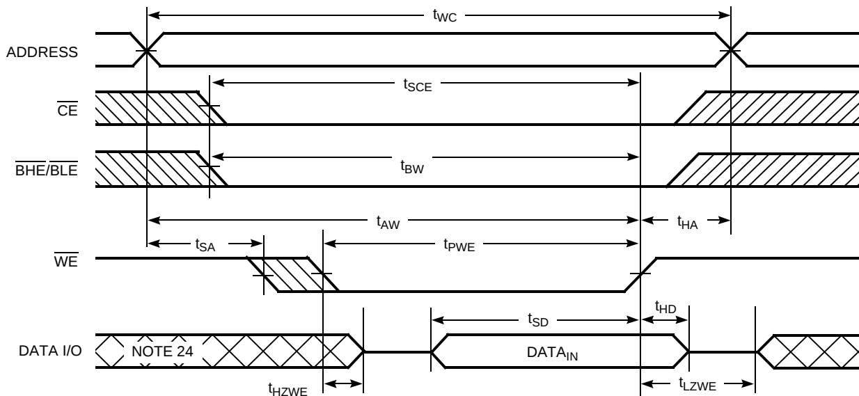
Figure 10. Write Cycle No. 4 ( \overline{\text{BHE/BLER}} controlled, \overline{\text{OE}} LOW) [23]
