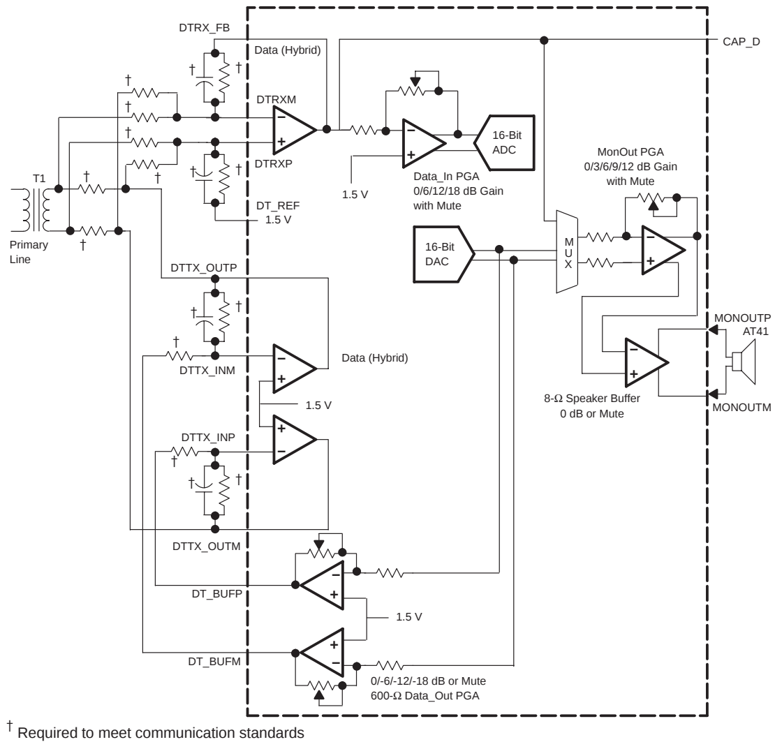
Figure 6–2. Differential Configuration Typical Application
