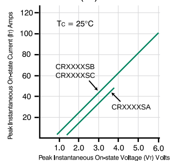
ON-STATE VOLTAGE ( V_T ) vs ON-STATE CURRENT ( I_T )
