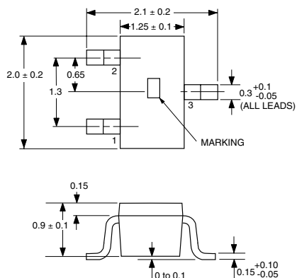
PACKAGE OUTLINE 30 (SOT-323)
