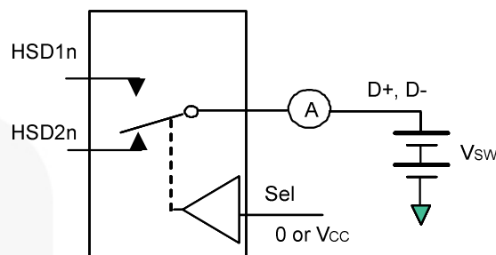
Figure 5. Off/On Leakage
