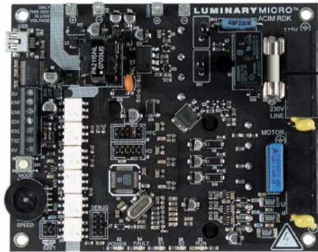
Figure 1. ACIM Control Board Only
