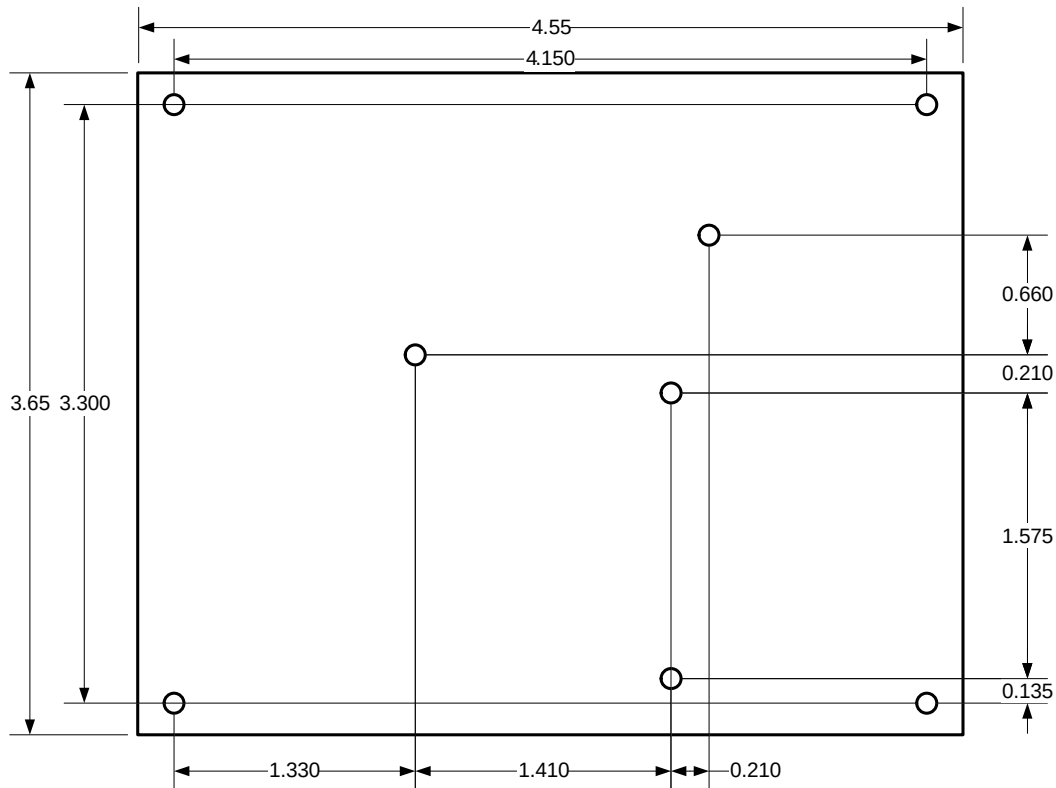
Figure 3. MDL-ACIM Mechanical Diagram
