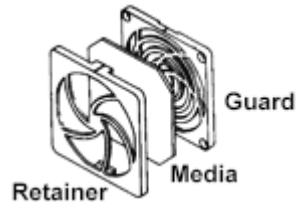
554141 Filter Guard Assembly
