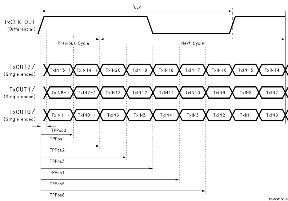
FIGURE 11. Transmitter LVDS Output Pulse Position Measurement
