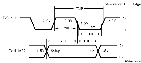
FIGURE 6. DS90C363A/DS90CF363A (Transmitter) Setup/Hold and High/Low Times (Falling Edge Strobe)
