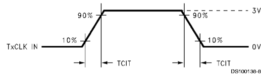
FIGURE 5. DS90C363A/DS90CF363A (Transmitter) Input Clock Transition Time
