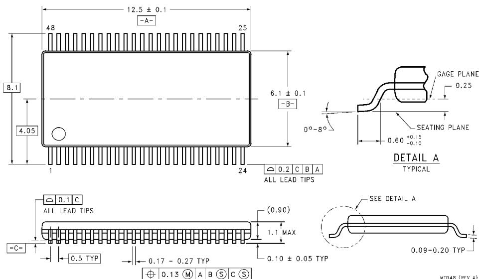
48-Lead Molded Thin Shrink Small Outline Package, JEDEC Order Number DS90C363AMTD, DS90CF363AMTD NS Package Number MTD48
