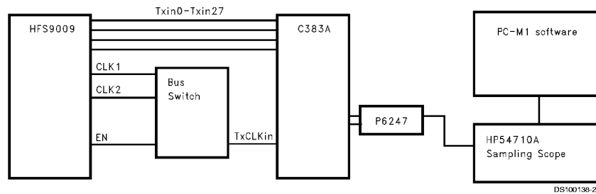
FIGURE 12. TJCC Test Setup
