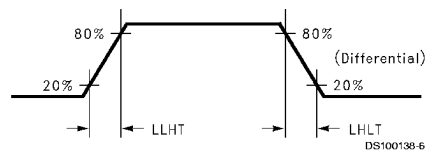
FIGURE 4. DS90C363A/DS90CF363A (Transmitter) LVDS Transition Times
