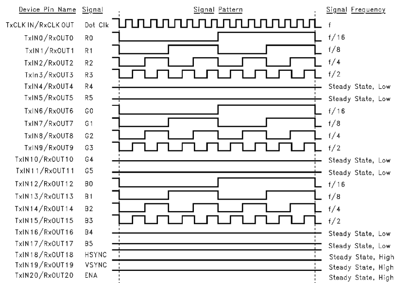
FIGURE 2. "16 Grayscale" Test Pattern (Notes 7, 8, 9, 10)
