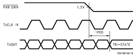
FIGURE 10. Transmitter Power Down Delay
