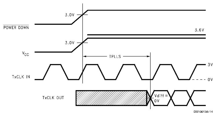
FIGURE 8. DS90C363A/DS90CF363A (Transmitter) Phase Lock Loop Set Time
