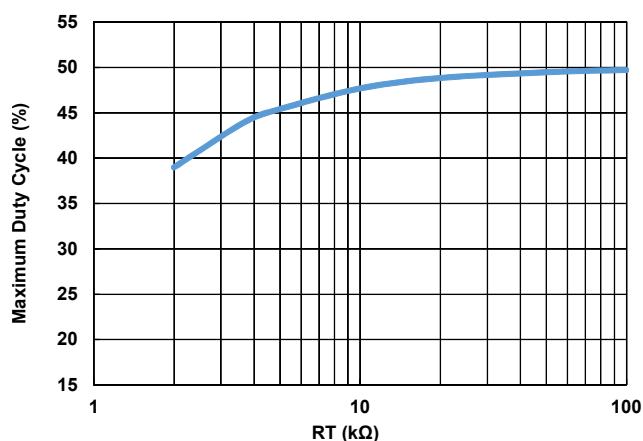
Figure 8. Maximum Duty Cycle vs RT (-50°C)
