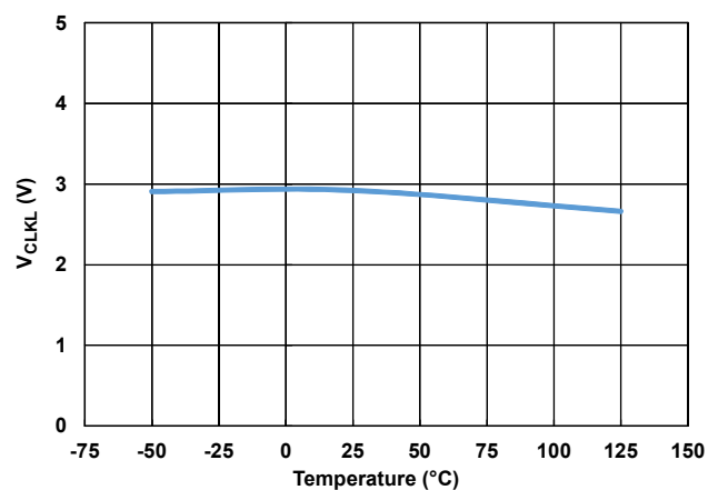
Figure 18. CT Peak Voltage vs Temperature
