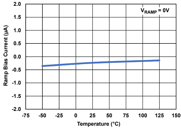
Figure 33. Ramp Bias Current vs Temperature
