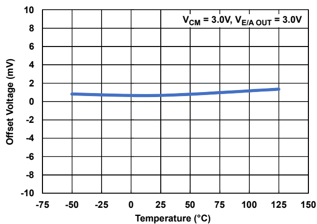
Figure 19. Error Amp V_{OS} vs Temperature
