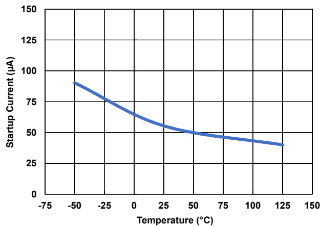
Figure 53. Startup Current vs Temperature
