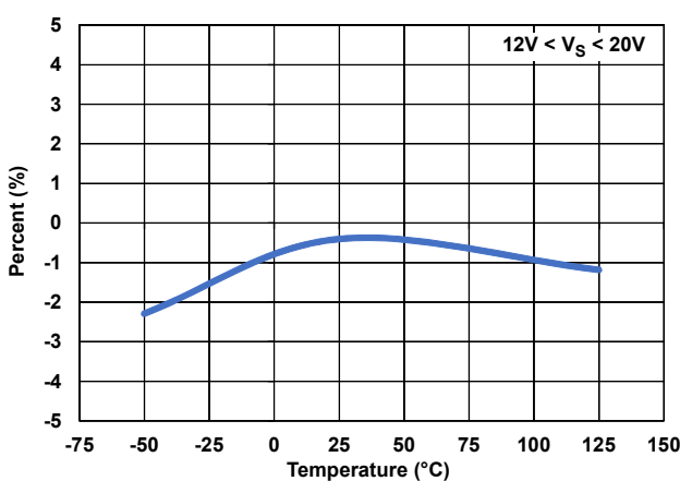
Figure 14. Oscillator Voltage Stability vs Temperature
