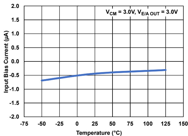
Figure 20. Error Amp I_{BIAS} vs Temperature
