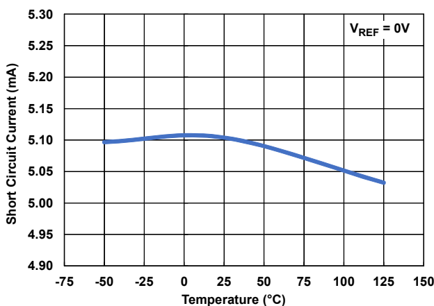
Figure 12. V_{REF} Short Circuit Current vs Temperature
