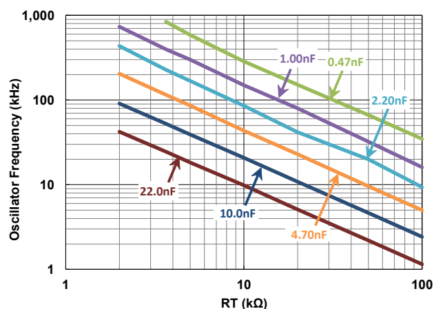
Figure 4. Oscillator Frequency vs RT and CT (+125°C)
