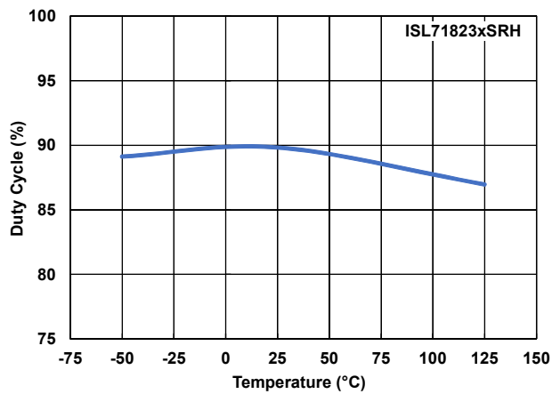
Figure 35. Maximum Duty Cycle vs Temperature
