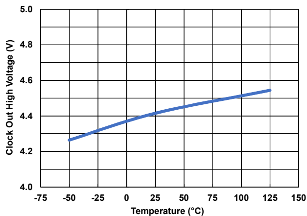
Figure 15. Oscillator V_{CLKH} vs Temperature
