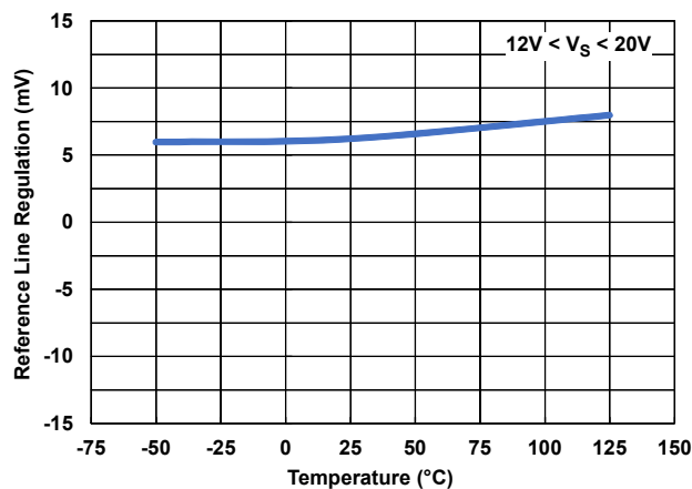
Figure 10. V_{REF} Line Regulation vs Temperature
