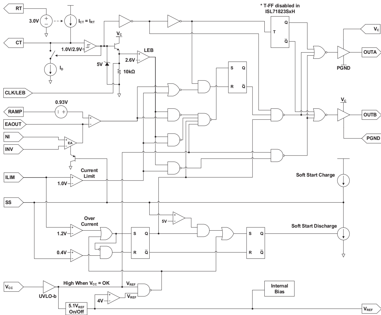
Figure 1. Block Diagram
