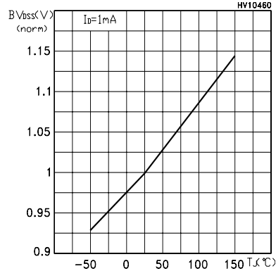
Figure 17: Normalized BV_{dss} vs Temperature
