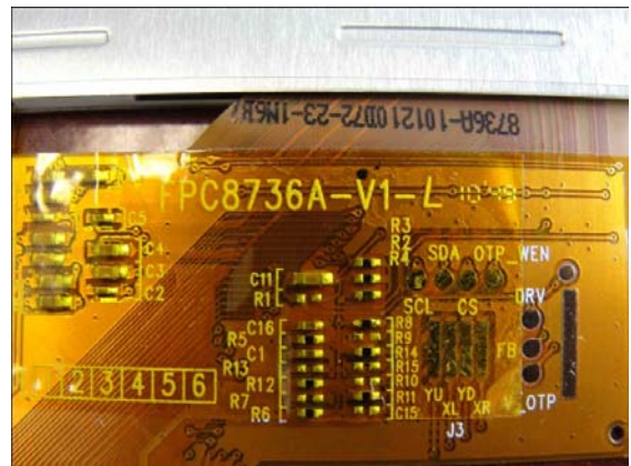
Resistor moved to position 8
