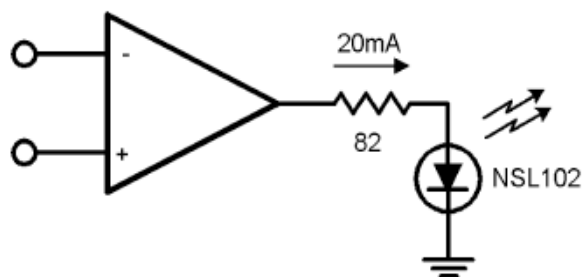
Figure 1. LED Driver
