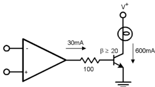
Figure 2. Lamp Driver
