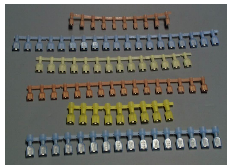
Quixon Fully-Insulated Quick-Disconnect Terminals (Red = 18 to 22 AWG; Blue = 14 to 16 AWG; Yellow = 10 to 12 AWG)
