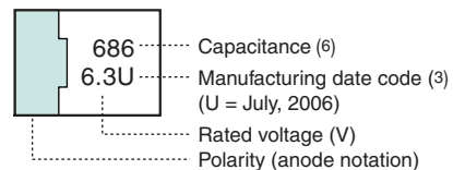
Cases B, C3, DL and D3
