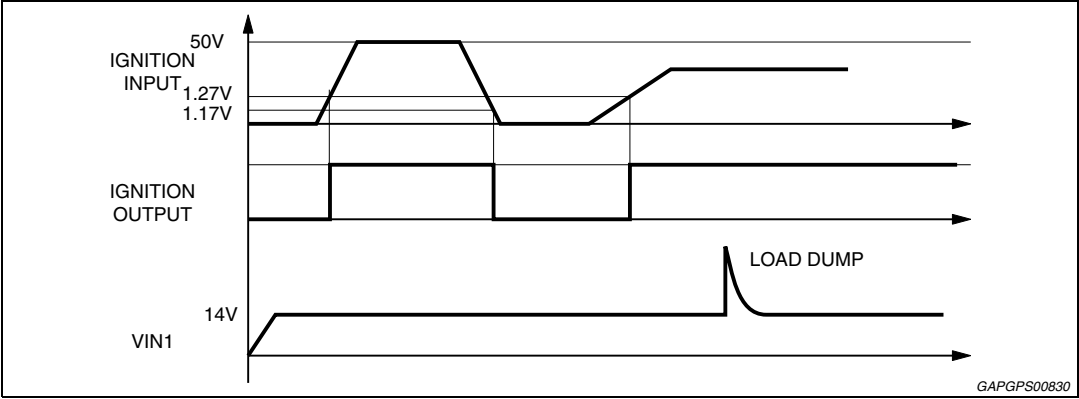
Figure 8. Ignition buffer diagram
