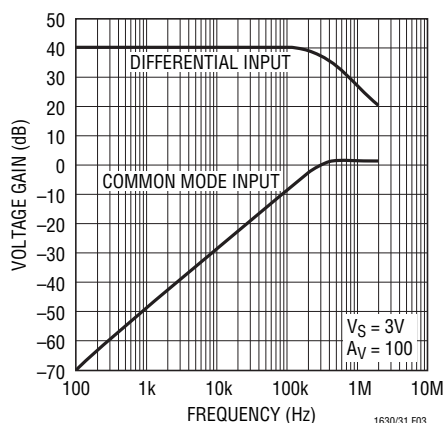
Figure 3. Frequency Response
