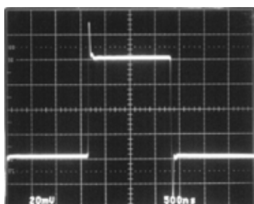
±15V Small-Signal Response
