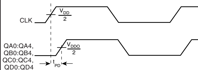
PROPAGATION DELAY
