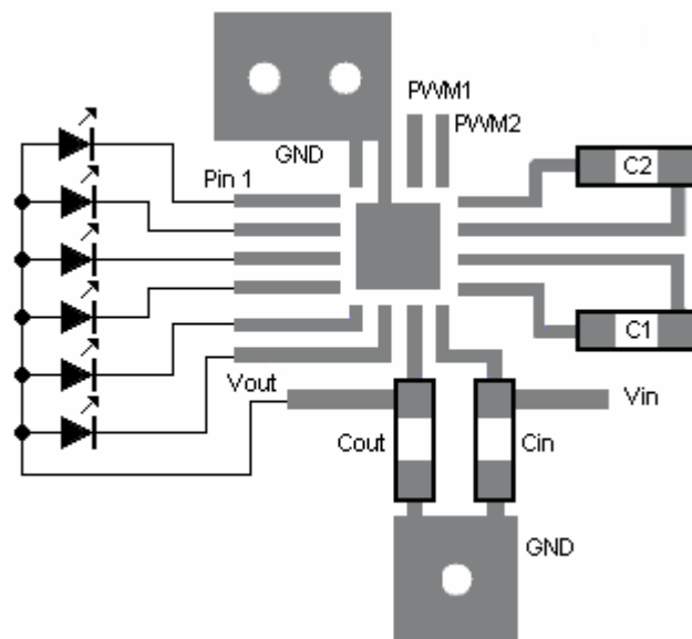
Figure 5. Recommended layout
