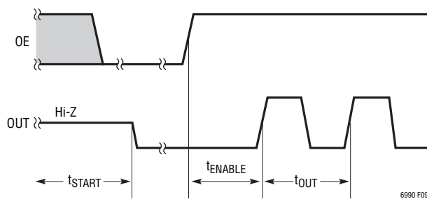
Figure 9. Start-Up Timing Diagram (OE = 0, N PIV = Any, Hi-Z = 0)
