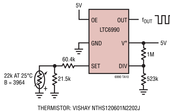
Temperature to Frequency Converter. 3% Linearity from -20°C ( f_{OUT} \approx 20\text{kHz} ) to 75°C ( f_{OUT} \approx 25\text{kHz} )
