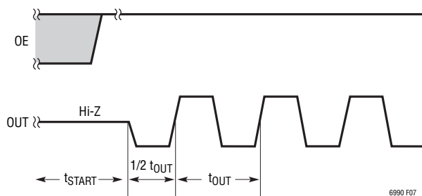
Figure 7. Start-Up Timing Diagram (OE = 1, N PIV = 1 or 2, Hi-Z = 0 or 1)
