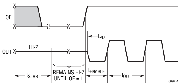
Figure 10. Start-Up Timing Diagram (OE = 0, N PIV = Any, Hi-Z = 1)
